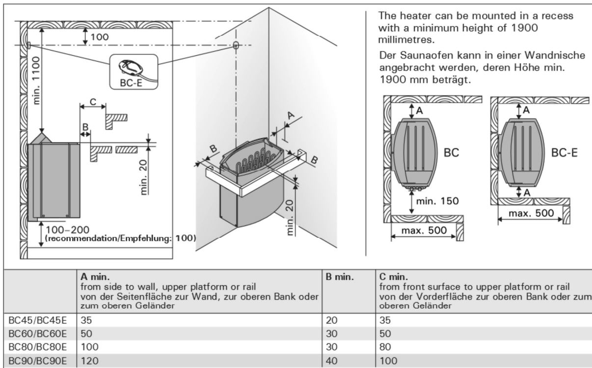
Figure 6. Safety distances (all dimensions in millimeters)
